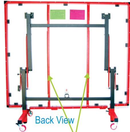
Patented Design 2+2 - 31 mm Steel Angle Unique Extra Back Supports for Warp Proof & Even Bounce
